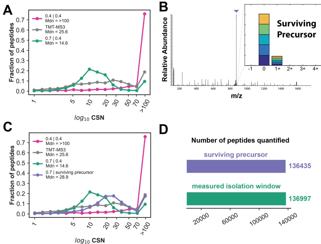
Figure 5. Incorporation of the surviving precursor monoisotopic envelope shape into the deconvolution algorithm increases robustness of TMTc+. A) Histograms of CSN of TMTc+ where the human / yeast standard was analyzed using different isolation windows on the instrument that are deconvolved using either proper or improper isolation window (IW) shapes (IW used on instrument | IW used during deconvolution). In the best case scenario for TMTc+, the narrowest isolation window (0.4 Th) is used and the shape of the 0.4 m/z isolation window is used during the deconvolution (pink, (0.4 Th | 0.4 Th)). To mimic a poorly calibrated instrument a 0.7 Th isolation window was used by the instrument, but the data was deconvolved assuming the shape of the isolation window was 0.4 Th (green (0.7 Th | 0.4 Th)). Shown for reference is the CSN for TMT-MS3 (grey). B) Representative MS2 spectra with a TMTc+ method. The tallest peak (purple arrow) is the “surviving precursor”, intact precursor from the MS1 that was not fragmented. Close inspection of the surviving precursor reveals that the ratios of each peak isolated from the pseudo-monoisotopic envelope in the MS1 (inset, colored bars) can be quantified. C) Same data as in A) but the same sample that was analyzed on the instrument with a 0.7 Th IW is now deconvolved using the ratios from the surviving precursor in the MS2 of each peptide instead of incorrectly assuming the isolation window used was the shape of 0.4 Th (purple (0.7 Th | surviving precursor)). An increase in CSN is observed. D) Number of peptides that are quantified from 24 90 minute reverse phase fractions using TMTc+ with either the surviving precursor approach (purple) or with the measured isolation window (green).
