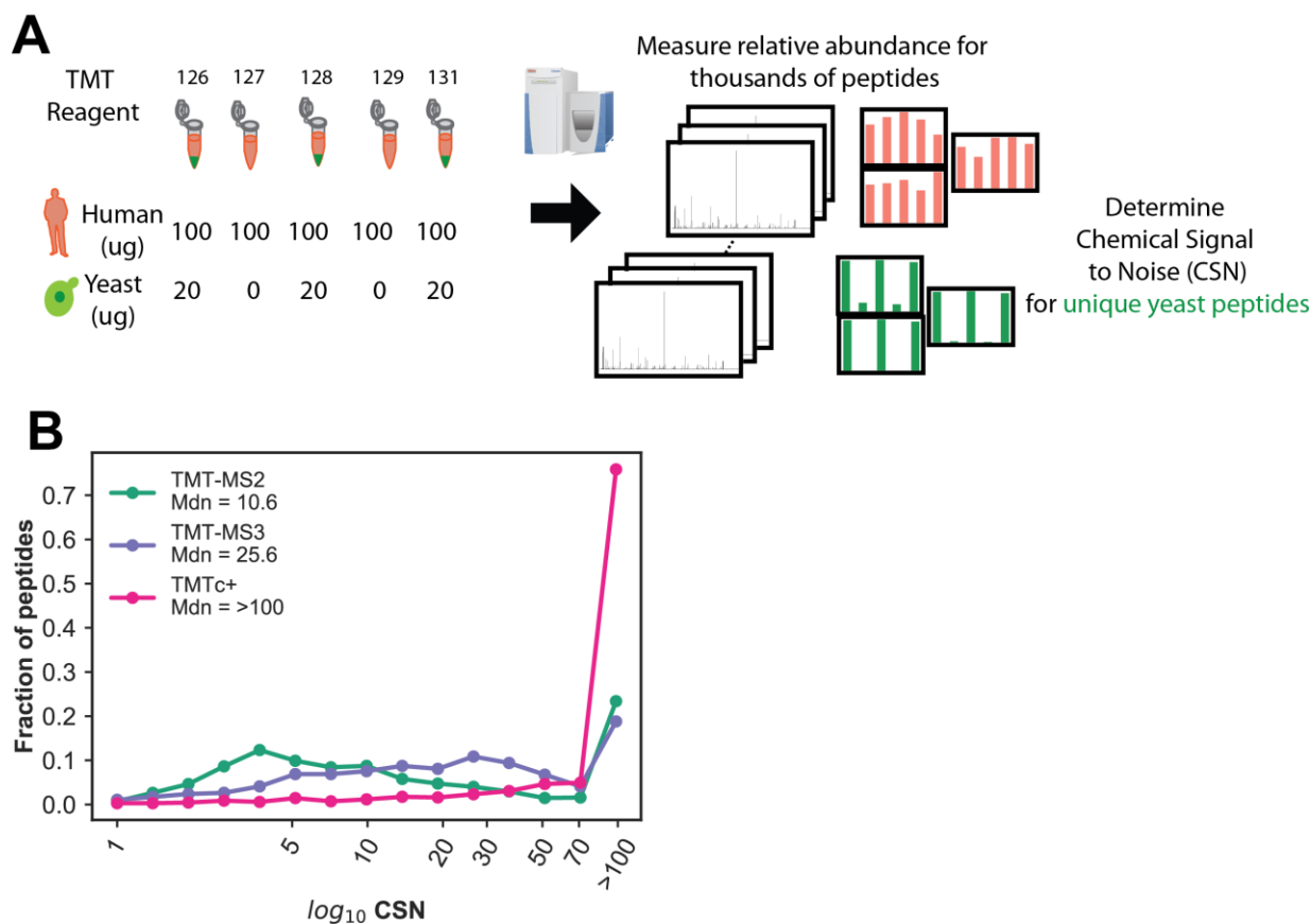
Figure 3. Signal to noise comparison between TMTc+, TMT-MS2, and TMT-MS3 A) A yeast / human standard was designed to assay the chemical signal to noise of TMTc+ relative to other multiplexed proteomics methods in use. Yeast (green) is only labeled with 3 of the 5 TMT reagents used, whereas human (pink) is labeled with all 5. The ratio of 126 TMT / 127 TMT for unique yeast peptides is used to assay the chemical signal to noise (CSN). A perfect measurement shows an infinite change. B) \log_{10} CSN histogram of unique yeast peptides using TMT-MS2, TMT-MS3, and TMTc+ from a 90 minute reverse phase fractionated sample. Bins are indicated with a circle. Due to restraints on ion counting statistics, any CSN larger than 100 was plotted as 100.
