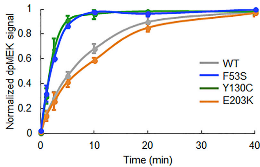
Figure 4. Quantification of MEK Activation by Raf via Western Blot Raf activates the F53S and Y130C variants more quickly than it activates the wild-type MEK and the E203K variant. The normalized dually phosphorylated (dp) MEK signal is an average of three experimental replicates, and the error bars represent the standard error of the mean.
