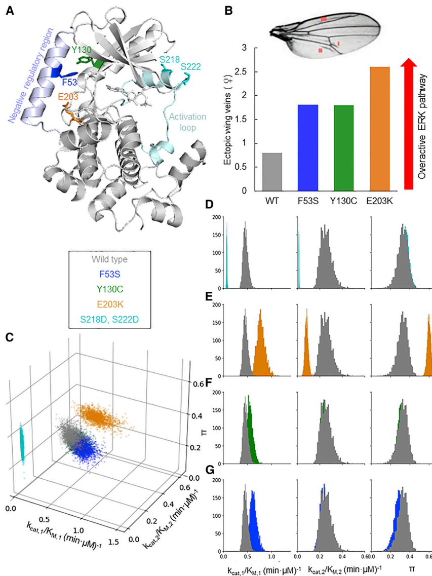
Figure 3. Mutations in MEK Can Be Categorized Based on Kinetic Parameters
