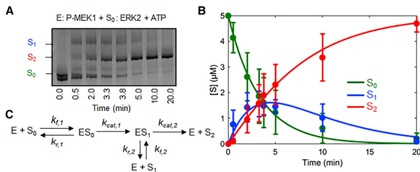
Figure 1. Determining Kinetic Parameters for MEK Activation of ERK
